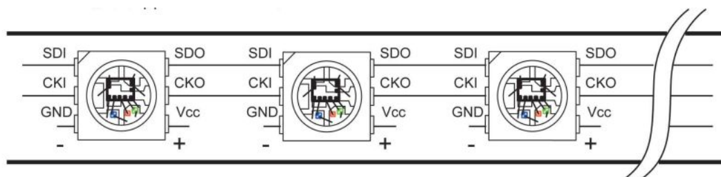
APA107 Chip
